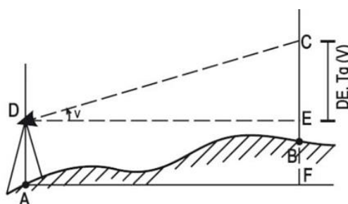
Figure 4: The settlement trigonometric
