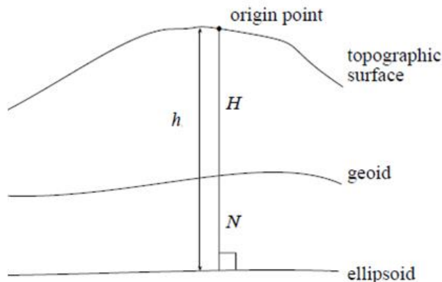
Figure 2: Elevation types and geoid diffraction
